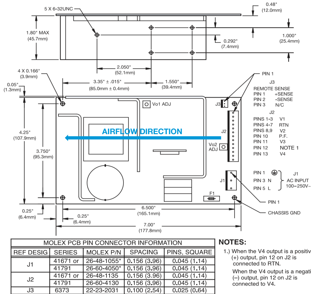
Figure 1. Mechanical Drawing
