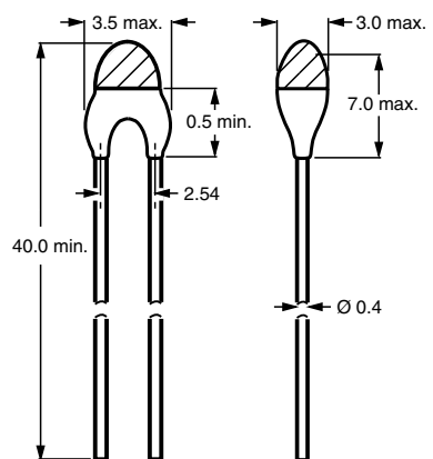
Component outline for 91152 to 91164
