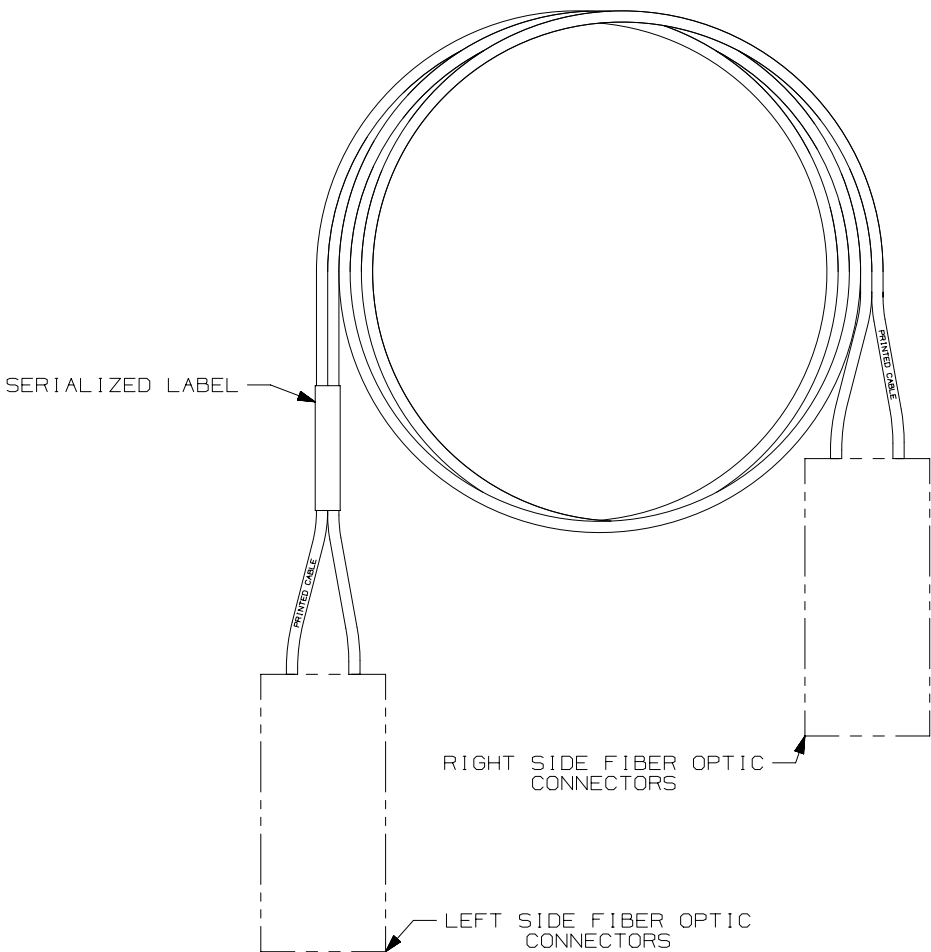
FOR 1.6mm/1.8mm/2.0mm/3.0mm DUPLEX PATCHCORD CABLE ASSEMBLIES
