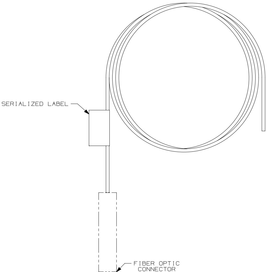
FOR 900um SIMPLEX PIGTAIL CABLE ASSEMBLIES
