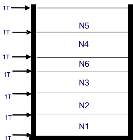
Figure 5—Winding Diagram
