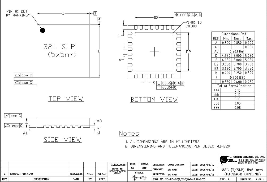
Figure 6-1. ESP8285 Package
