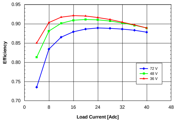
Figure 2.5V.11. Efficiency vs. load current and input voltage for QME48T40025 converter mounted horizontally with air flowing from pin 1 to pin 3 at a rate of 300 LFM (1.5 m/s) and T_a = 25^{\circ}\text{C} .
