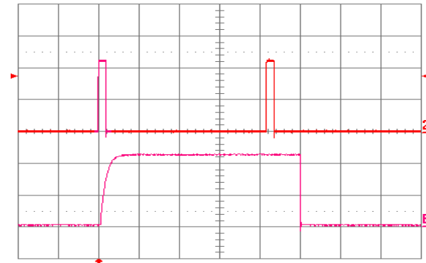
Figure 1.5V.24. Load current (top trace, 20 A/div., 50 ms/div.) into a 10 \text{ m}\Omega short circuit during restart, at V_{in} = 48 \text{ V} . Bottom trace (20 A/div., 2 ms/div.) is an expansion of the on-time portion of the top trace.
