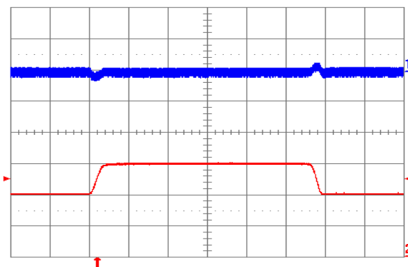
Figure 1.0V.17. Output voltage response to load current step-change (20 A – 30 A – 20 A) at V_{in} = 48\text{ V} . Top trace: output voltage (100 mV/div.). Bottom trace: load current (10 A/div.). Current slew rate: 0.1 A/ \mu\text{s} . C_o = 1\text{ }\mu\text{F} ceramic. Time scale: 0.2 ms/div.
