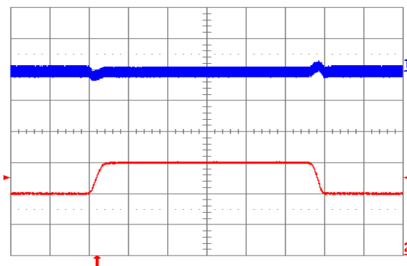
Figure 1.5V.17. Output voltage response to load current step-change (20 A - 30 A - 20 A) at V_{in} = 48\text{ V} . Top trace: output voltage (100 mV/div.). Bottom trace: load current (10 A/div.). Current slew rate: 0.1 A/ \mu\text{s} . C_o = 1\text{ }\mu\text{F} ceramic. Time scale: 0.2 ms/div.
