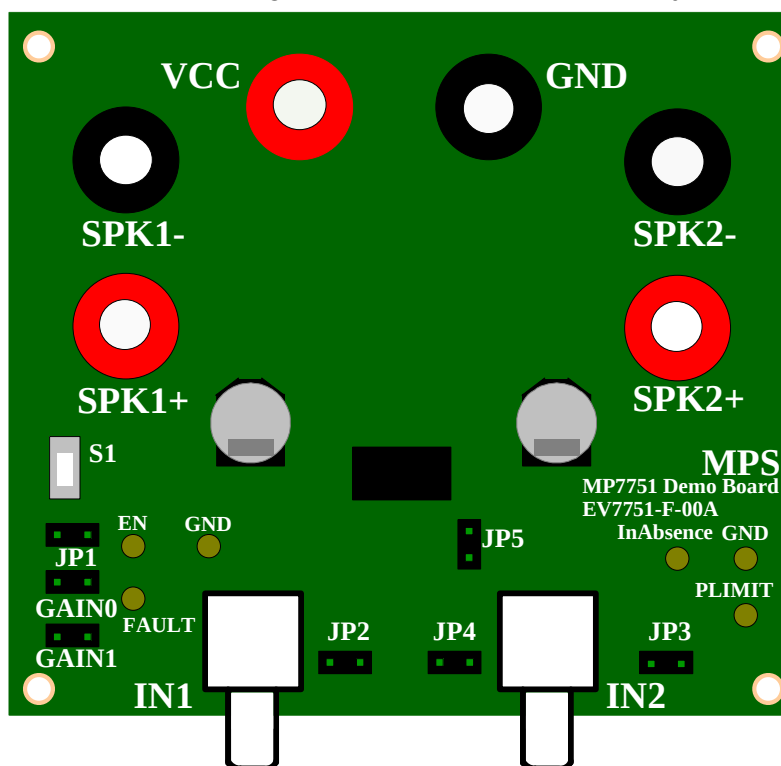
Figure 5—EV7751-F-00A Connection Diagram
