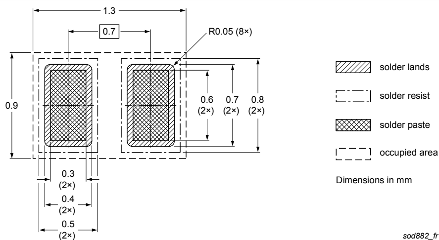
Figure 5. Reflow soldering footprint SOD882
