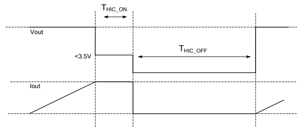
Figure 7: Over-Current Protection
