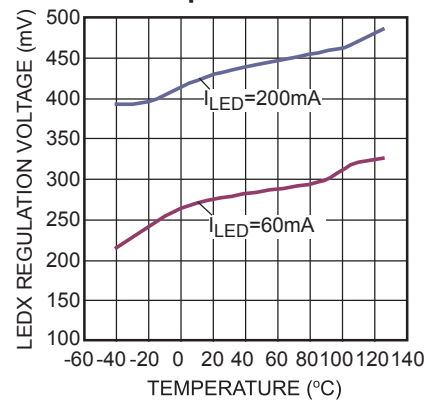
LEDX Regulation Voltage vs. Temperature
