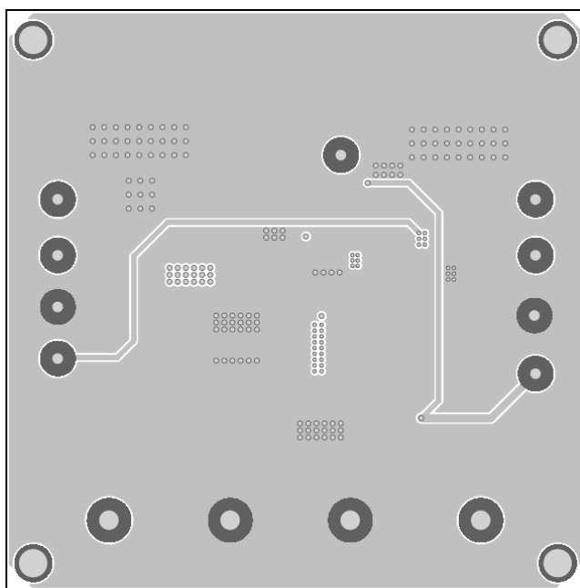
Figure 4—Inner Layer2
