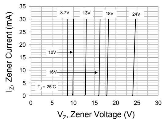
Fig.6 Typical Zener Characteristics
