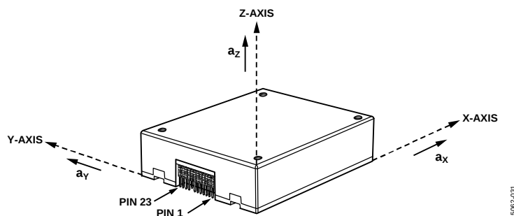
Figure 35. Accelerometer Axis and Polarity Assignments
