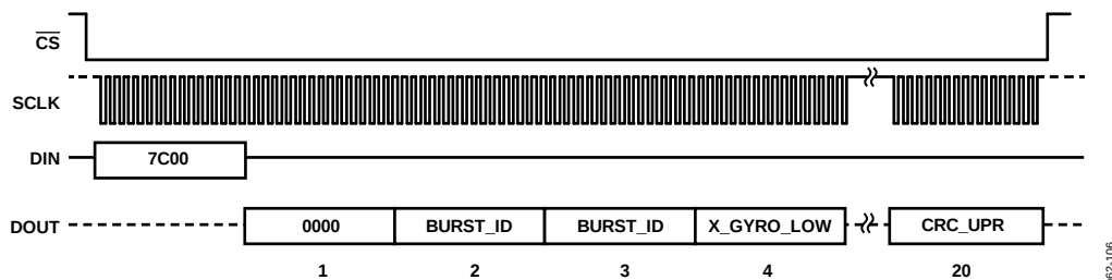
Figure 6. Burst Read Function Sequence Diagram, 20 Segments
