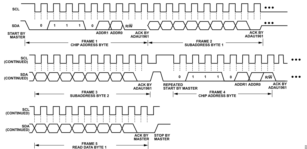
Figure 49. I 2 C Read from ADAU1961 Clocking
