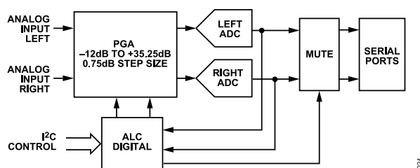
Figure 36. ALC Architecture
