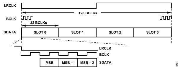
Figure 60. TDM 4 Mode
