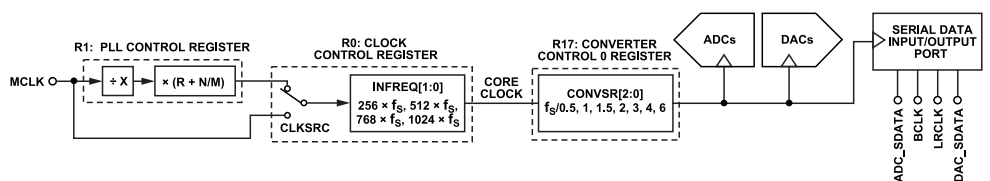
Figure 29. Clock Tree Diagram
