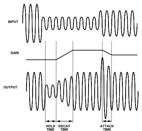
Figure 37. Basic ALC Operation
