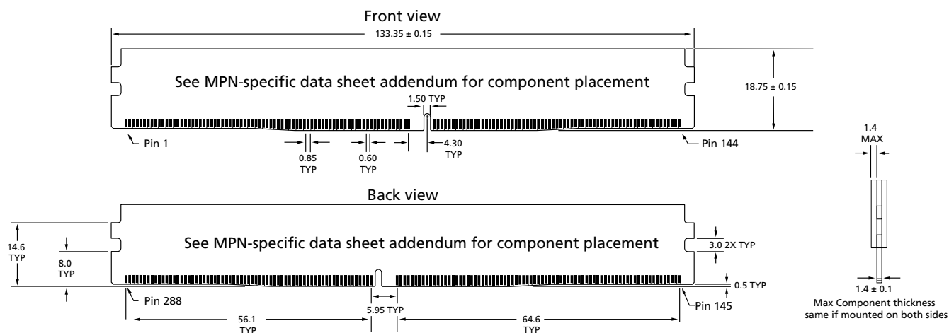
Figure 2: 288-Pin DDR4 VLP RDIMM
