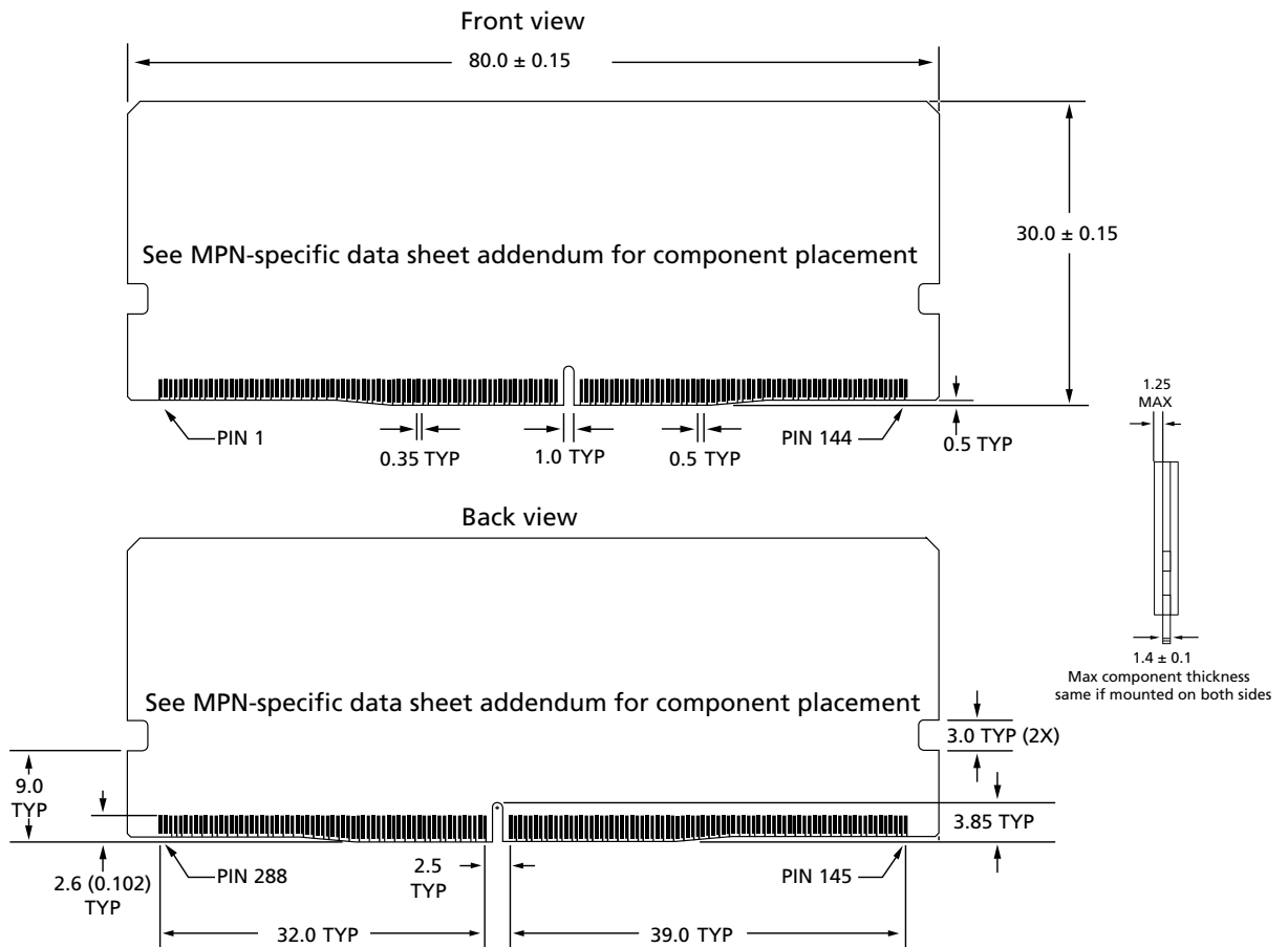
Figure 3: 288-Pin DDR4 MiniRDIMM
