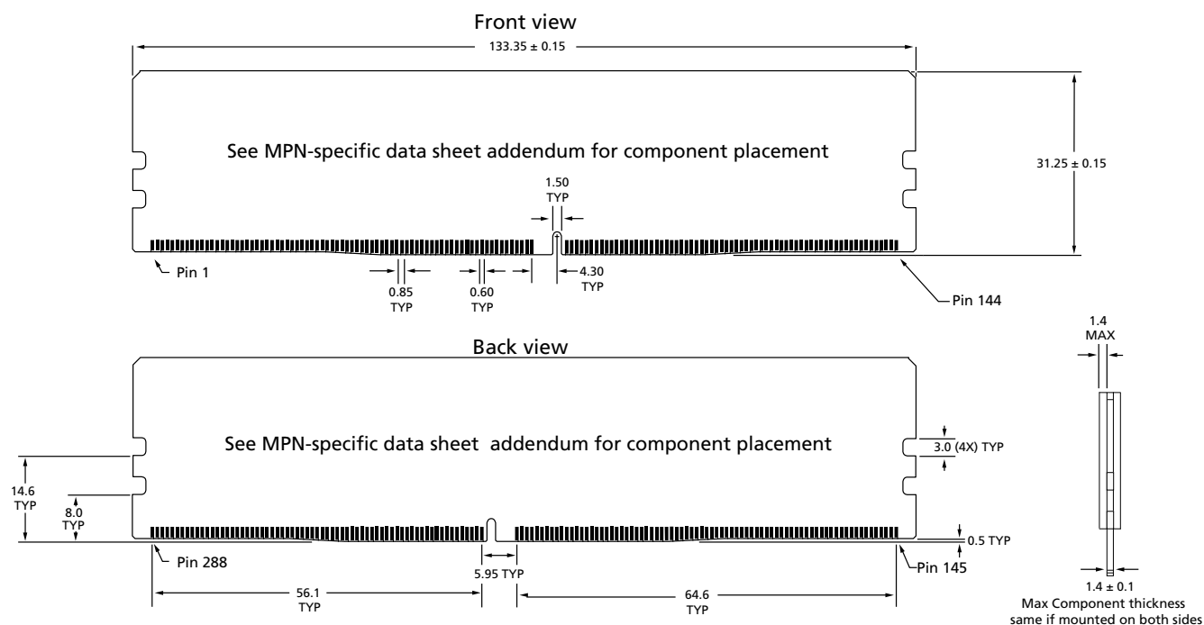
Figure 1: 288-Pin DDR4 RDIMM
