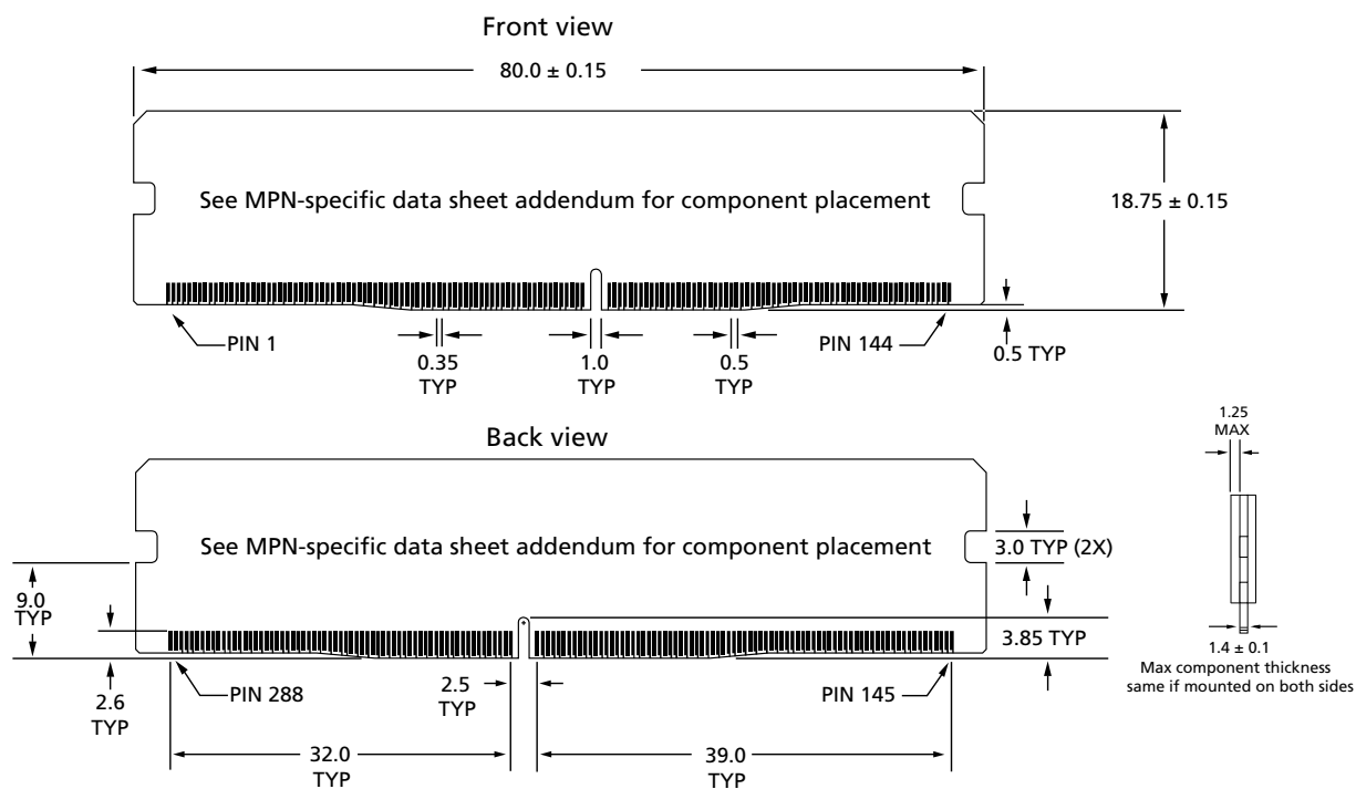
Figure 4: 288-Pin DDR4 VLP MiniRDIMM
