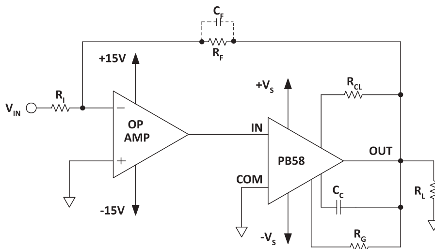
Figure 16: Typical Application
