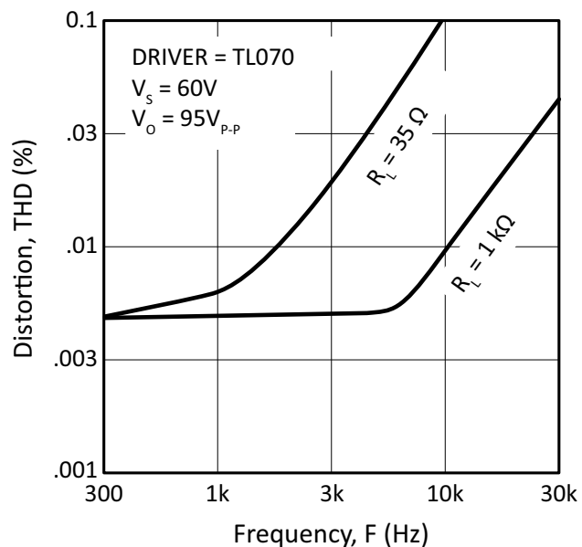
Figure 14: Harmonic Distortion
