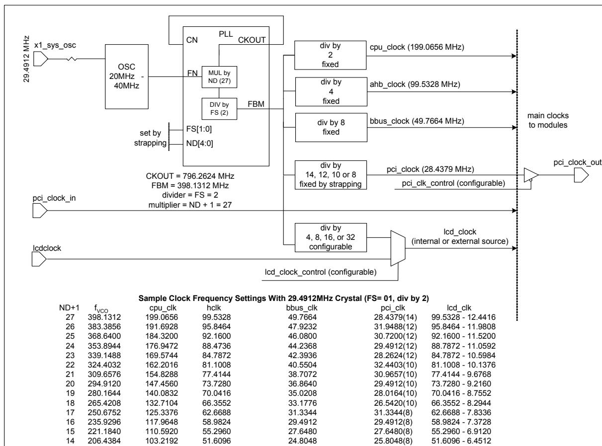
Figure 3: NS9750B-A1 system clock generation (PLL)
