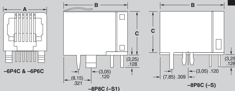
–8P8C (–S1)
