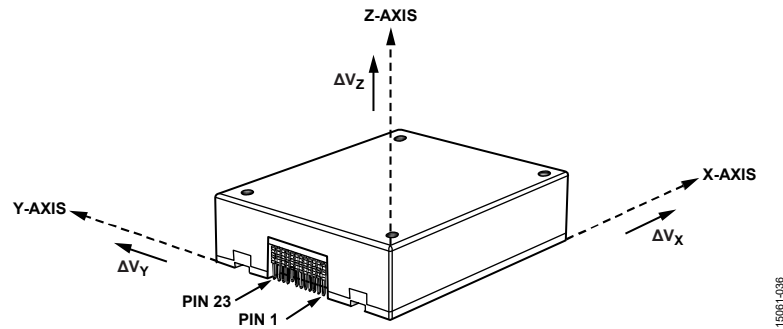
Figure 44. Delta Velocity Axis and Polarity Assignments
