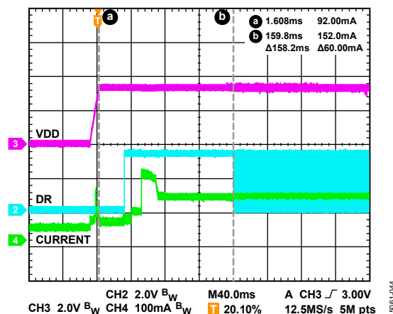
Figure 52. Transient Current Demand, Startup
