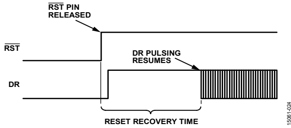
Figure 32. Data Ready Response During Reset ( \overline{RST} = 0 ) Recovery
