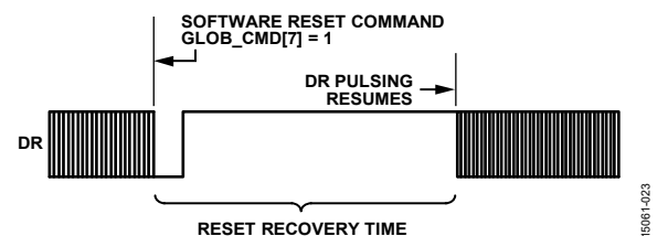
Figure 31. Data Ready Response During Software Reset (Register GLOB_CMD, Bit 7 = 1) Recovery
