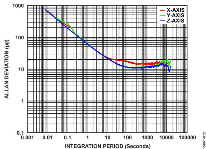
Figure 12. Accelerometer Allan Deviation
