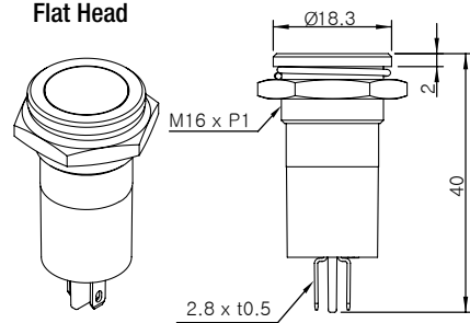
Flat Head
