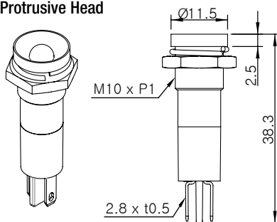
Protrusive Head
