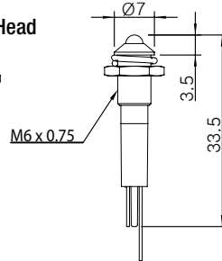
Round Head
