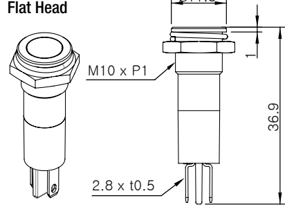
Flat Head
