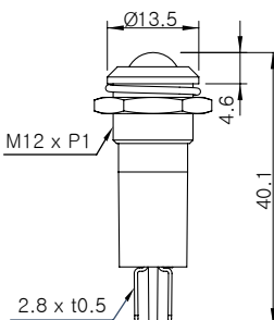
Round Head
