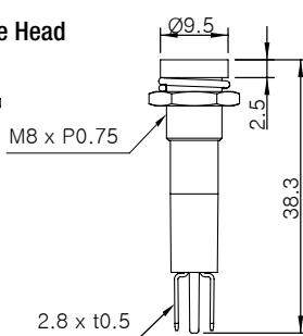
Protrusive Head
