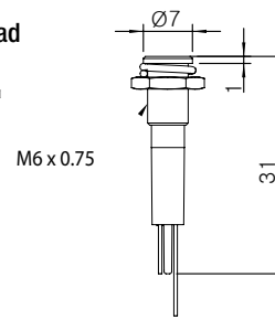
Flat Head
