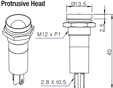
Protrusive Head
