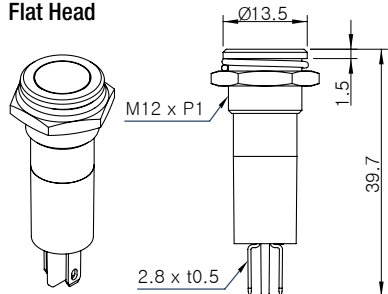
Flat Head
