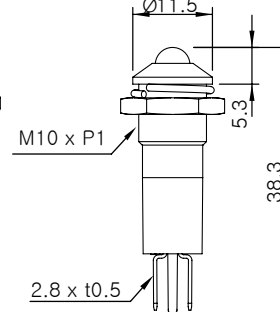
Round Head
