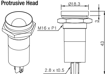
Protrusive Head
