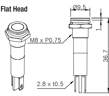
Flat Head
