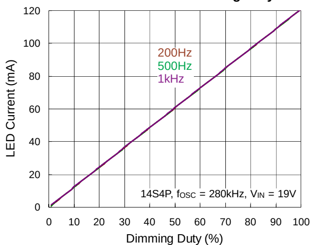
LED Current vs. Dimming Duty
