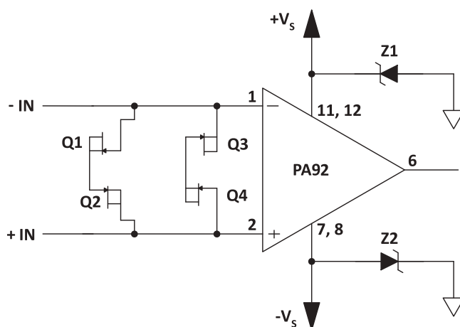
Figure 15: Overvoltage Protection
