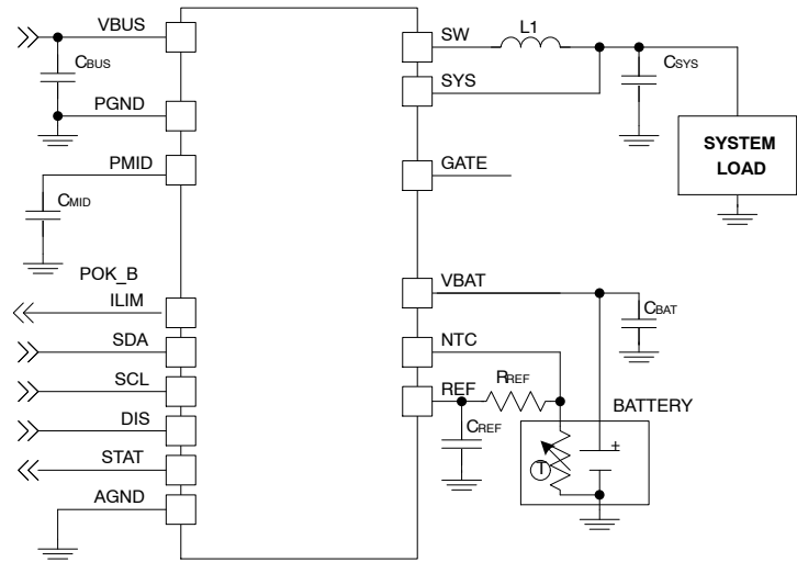
Figure 1. Typical Application
