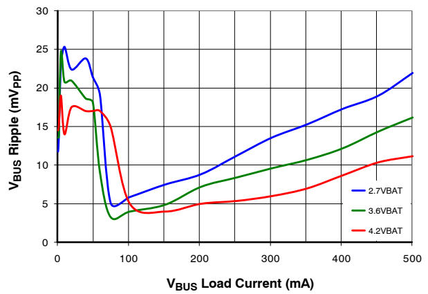
Figure 26. Output Ripple vs. I_{BUS} over V_{BAT}
