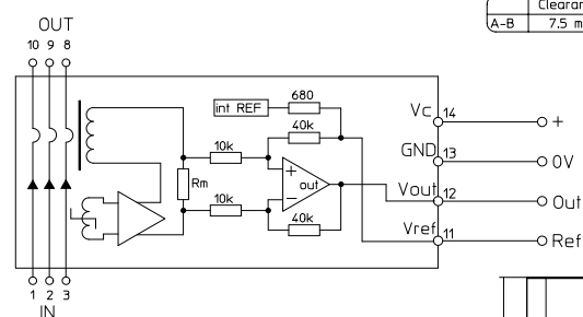
Connection
