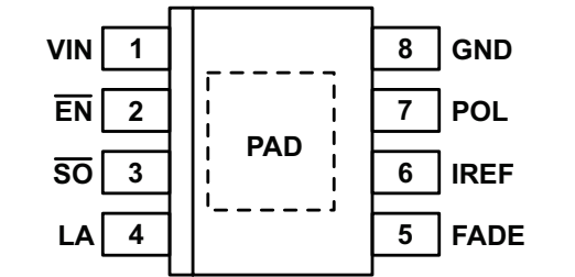
Package LJ, 8-Pin SOICN Pinout Drawing
