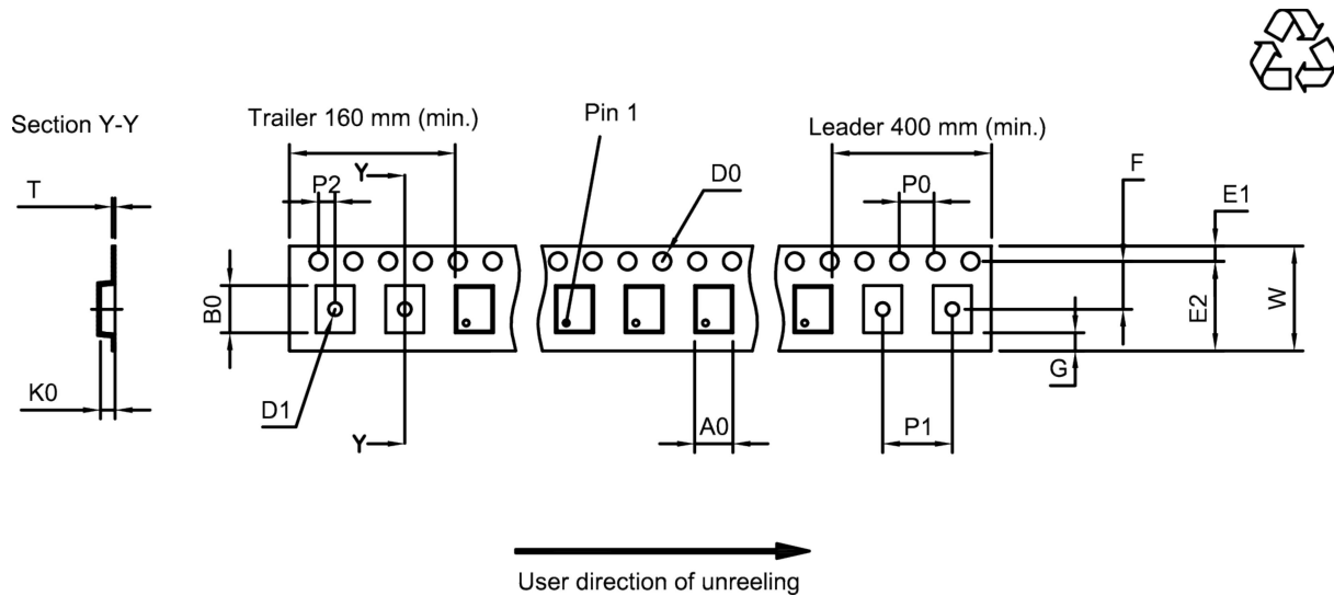
Figure 6: Drawing of tape (first-angle projection) for illustration only and not to scale. The valid tape dimensions are listed in Table 1.
