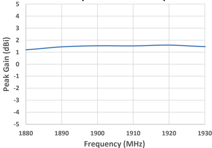
Gain (1880 – 1930 MHz)
