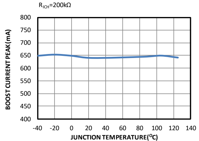
Boost switching Peak Current vs. Temperature
