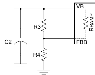
Figure 15: VB Regulation Feedback Circuit
