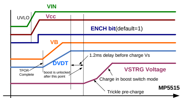
Figure 3: System Power-Up Sequence
