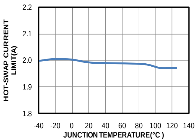
Hot-Swap Current Limit vs. Temperature
