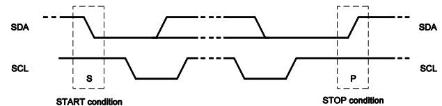
Figure 10: Start and Stop Conditions
