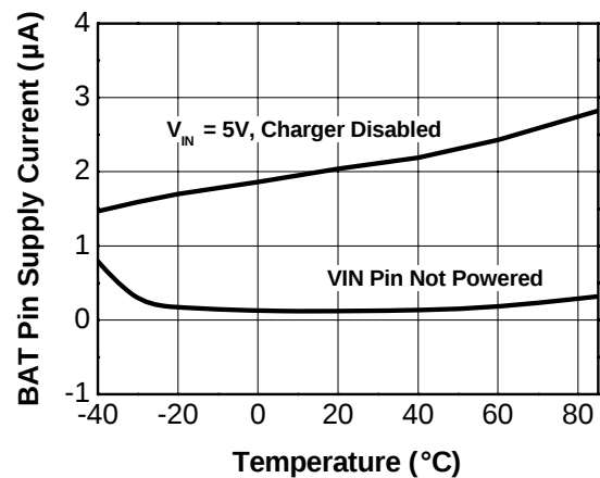
Figure 15. BAT Pin Supply Current vs Temperature I_{CHG} = 650 mA, V_{BAT} = 5.0 V
