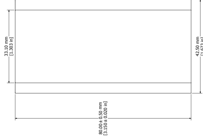
EXTRUSION PROFILE
