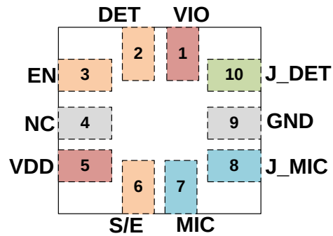
Figure 3. Pin Assignment (Through View)
