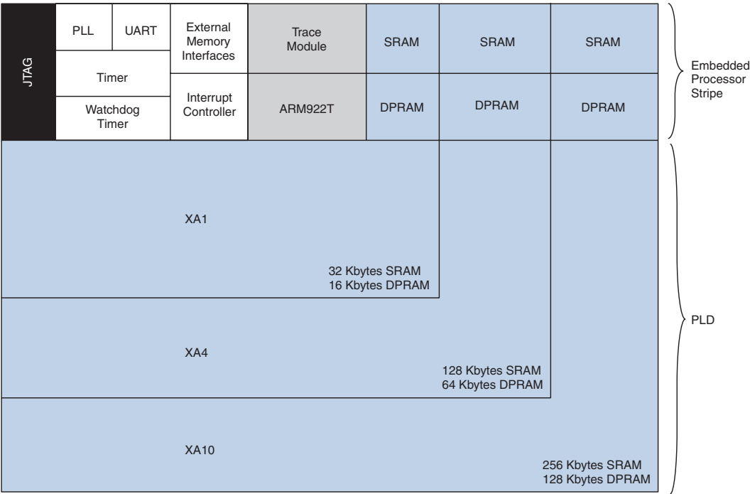
Figure 1. Excalibur Architecture
