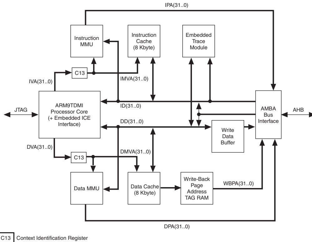
Figure 3. ARM922T Embedded Processor Internal Organization
