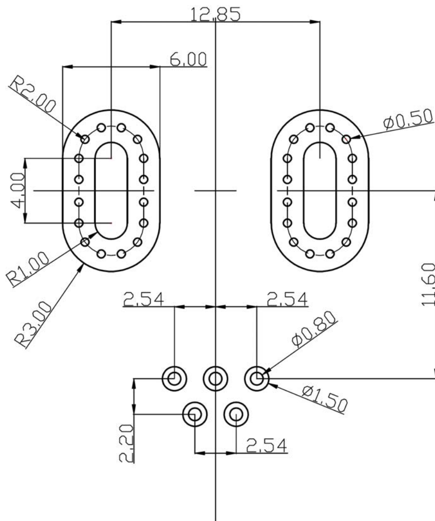
Figure 10. Recommended land pattern of CQ-2065
