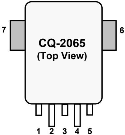
Figure 3. Pin-out diagram
