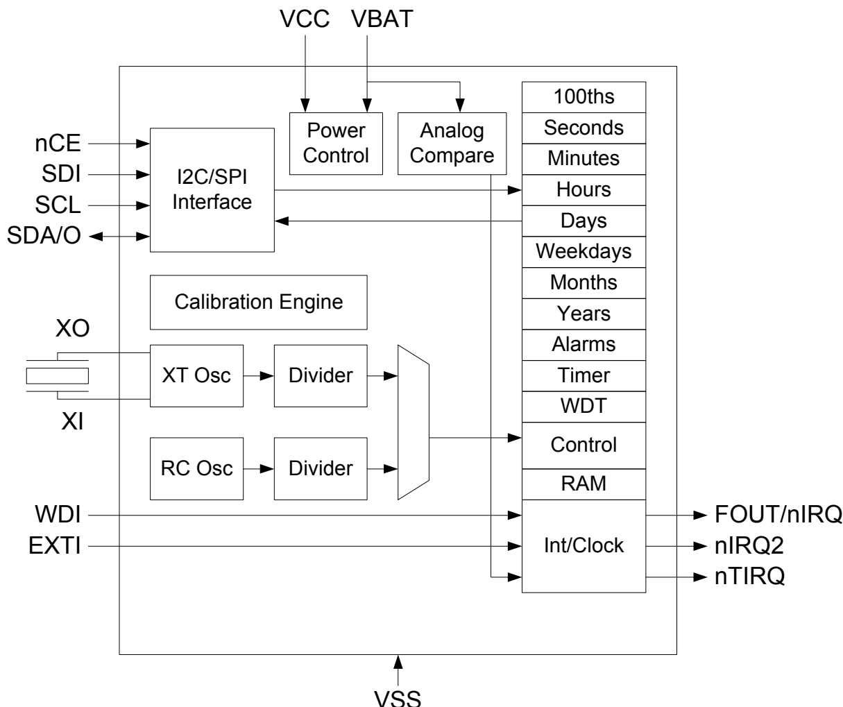
Figure 22. Detailed Block Diagram
