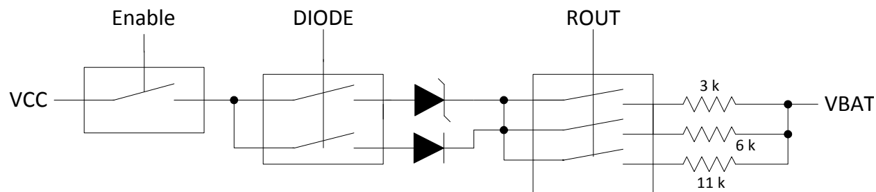
Figure 33. Trickle Charger
