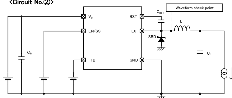
<Circuit No.②>
