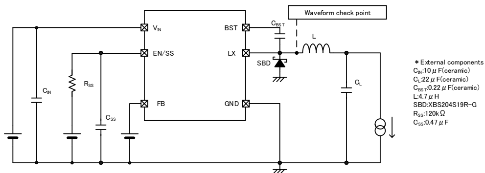
<Circuit No.⑤>
