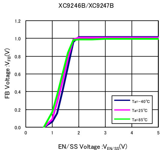
(13) FB Voltage vs. EN/SS Voltage
