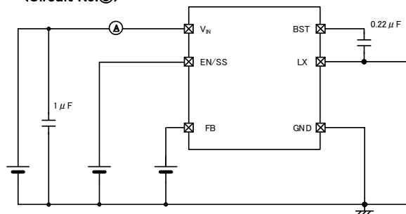
<Circuit No.③>
