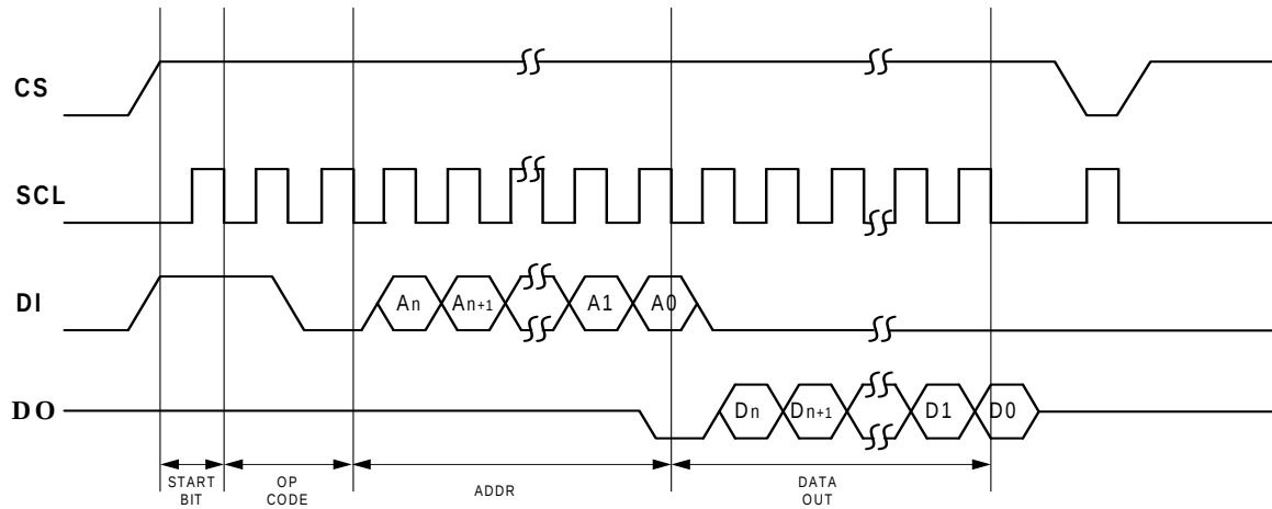
READ Timing
