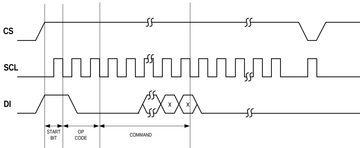
EWEN Timing
