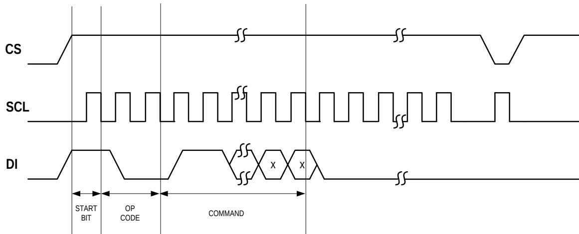
EWEN Timing
