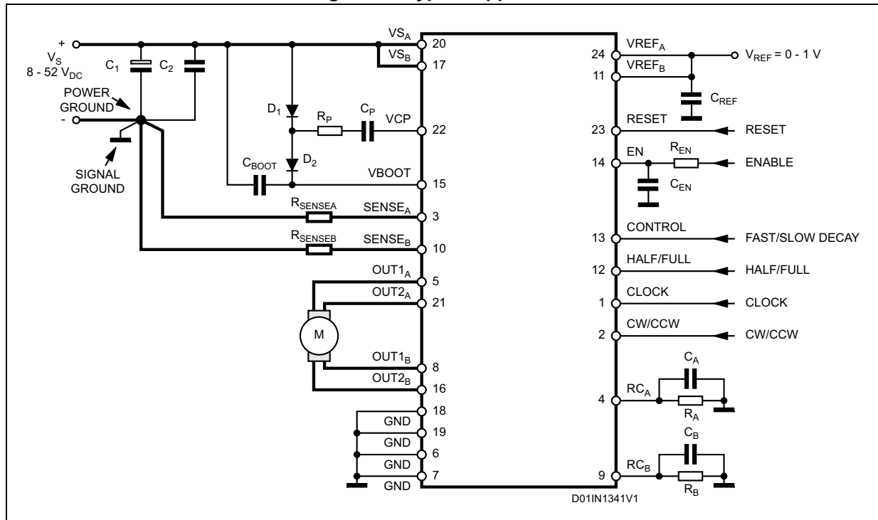
Figure 25. Typical application
