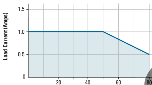
AMBIENT TEMPERATURE (°C) Max. Load Current vs. Temp.
