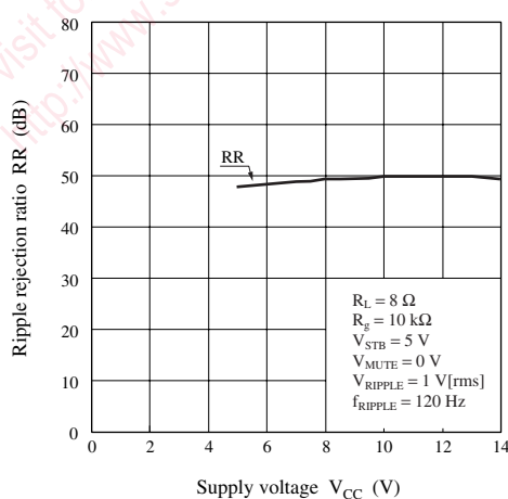
RR — V_{CC}
