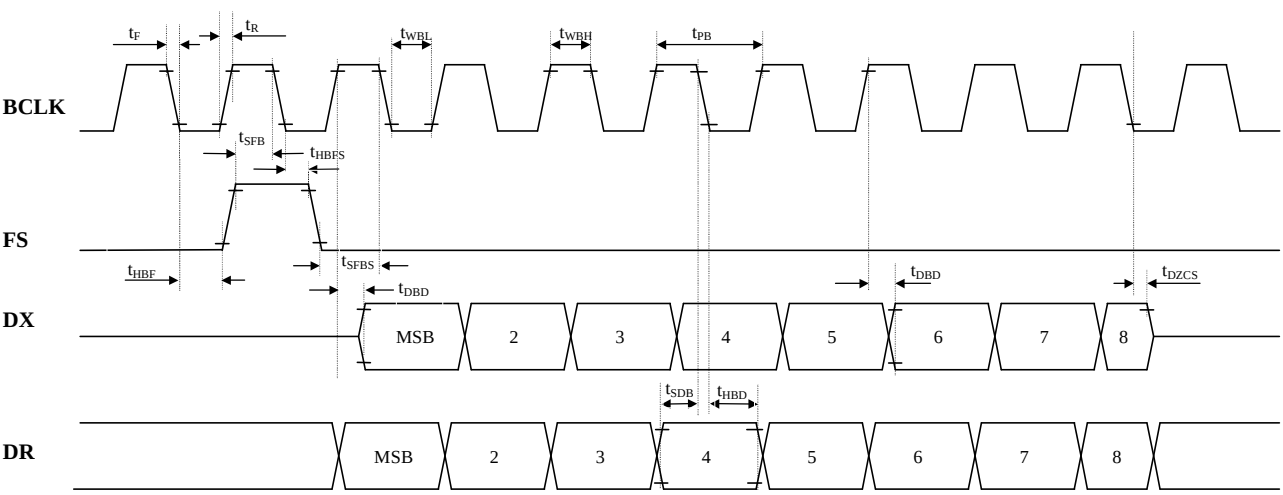
図 2 PCM Interface Timing < Short Frame >
