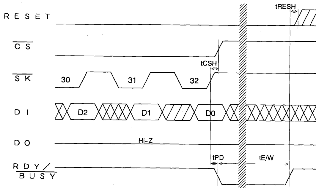
Ready / BUSY Signal Output ( R D Y / \overline{B U S Y} pin)
