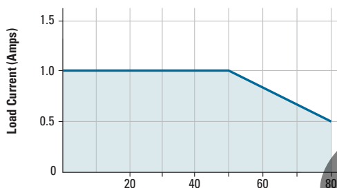
AMBIENT TEMPERATURE (°C) Max. Load Current vs. Temp.
