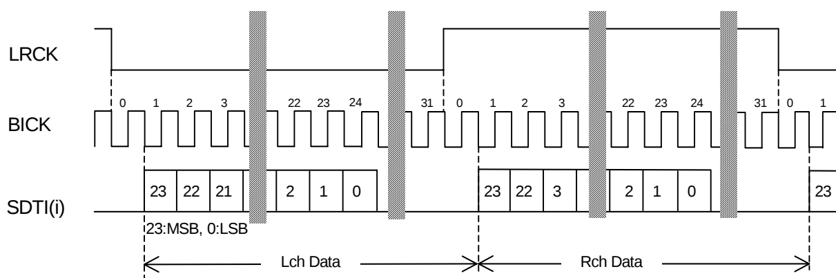
Figure 13. Mode 5/7 Timing
