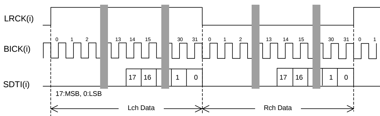
Figure 9. Mode 1 Timing
