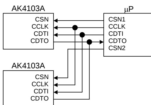
Figure 20. Typical connection with \mu P
