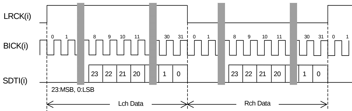
Figure 11. Mode 3 Timing
