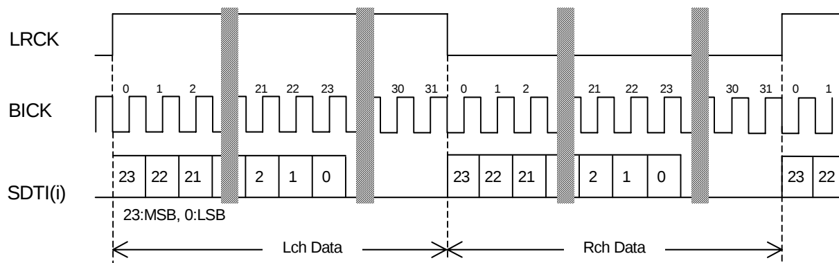
Figure 12. Mode 4/6 Timing
