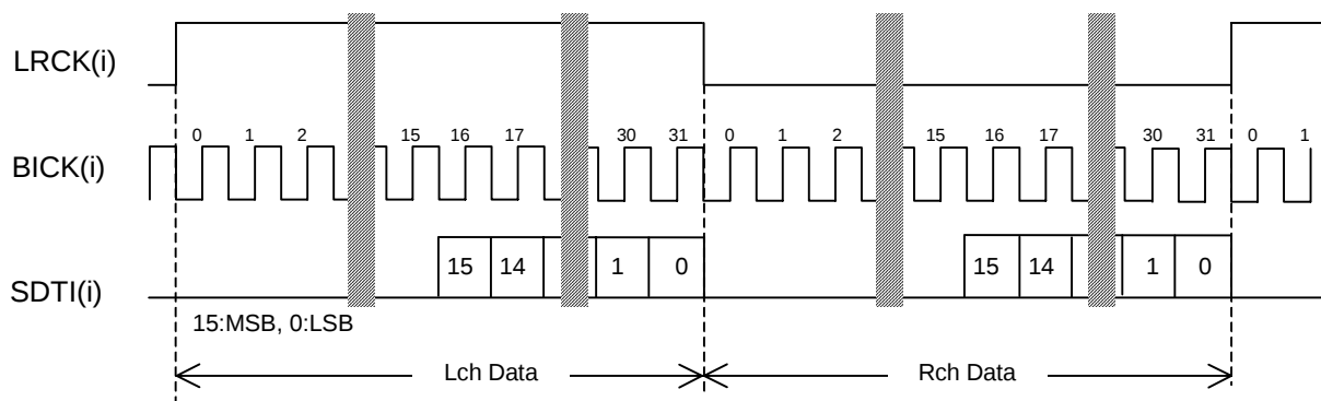
Figure 8. Mode 0 Timing
