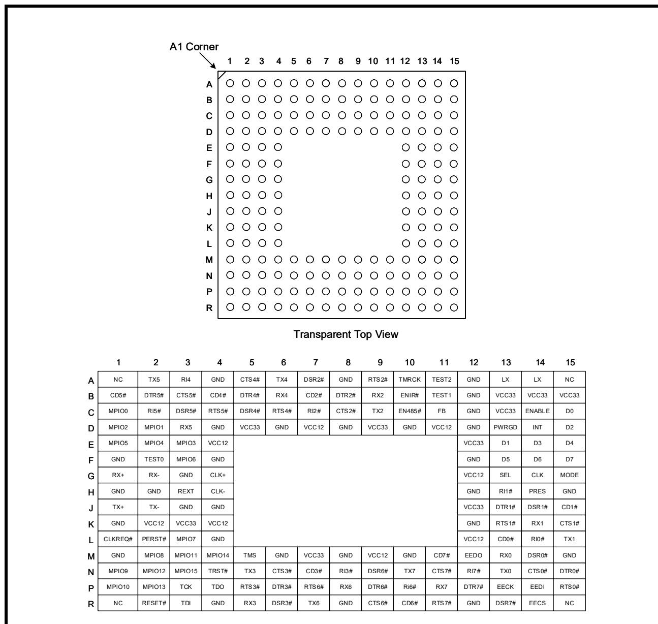
FIGURE 2. 176-FPBGA PINOUT
