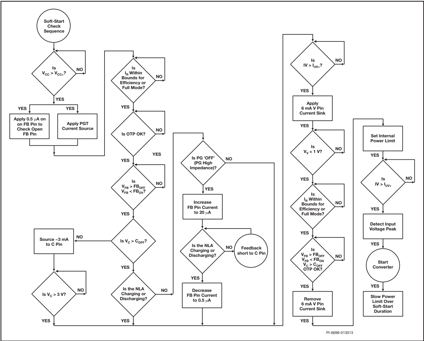
Figure 8. Start-Up Sequence.
