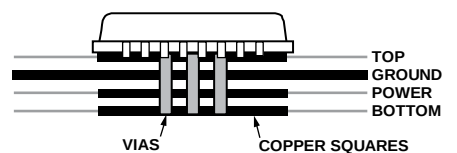
Figure 65. Exposed Pad Layout Example, Side View
