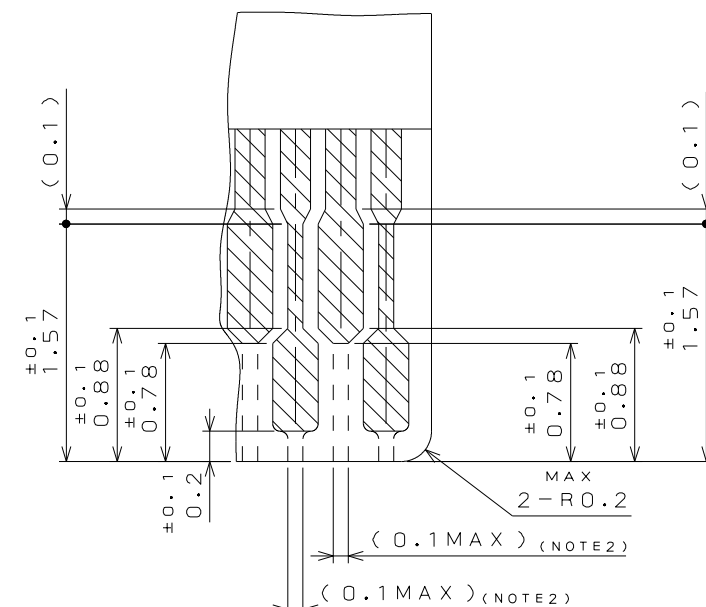
DETAIL C (SCALE 20:1)
