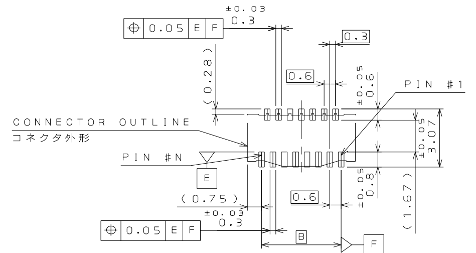
APPLICABLE P.C.B. DIMENSION (REF.) (SCALE 5:1)
