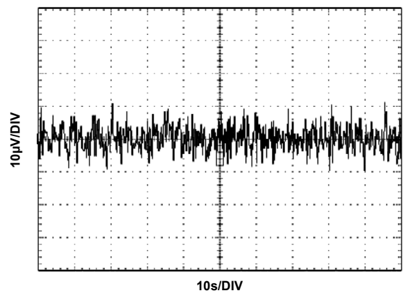
FIGURE 41. V_{OUT} NOISE
