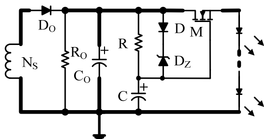
Figure9: Ripple Suppressor
