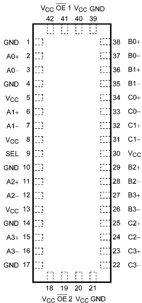
TC7PCI3412MT
